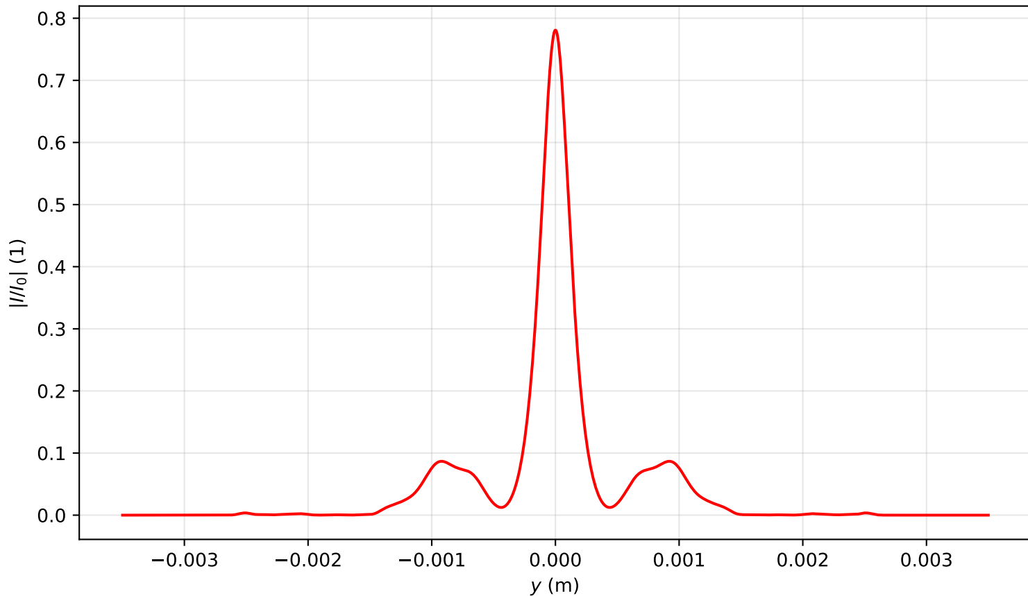
Intensity profile I(x=0, y, z=1.911)/I_0 , P_{in}=8.5P_{cr} , artificial time
